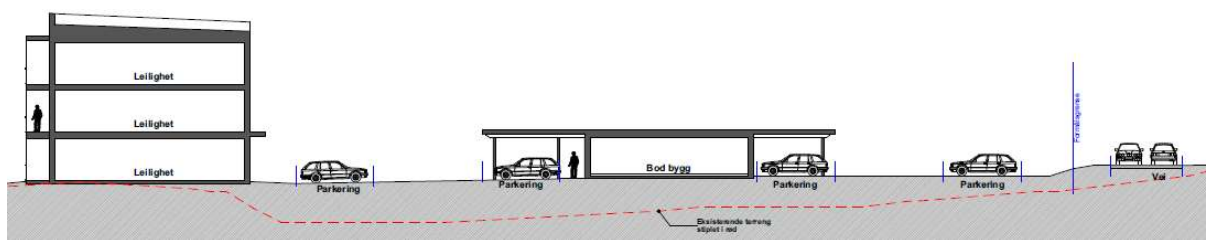
Figur 19. Snitt A. Norconsult AS
